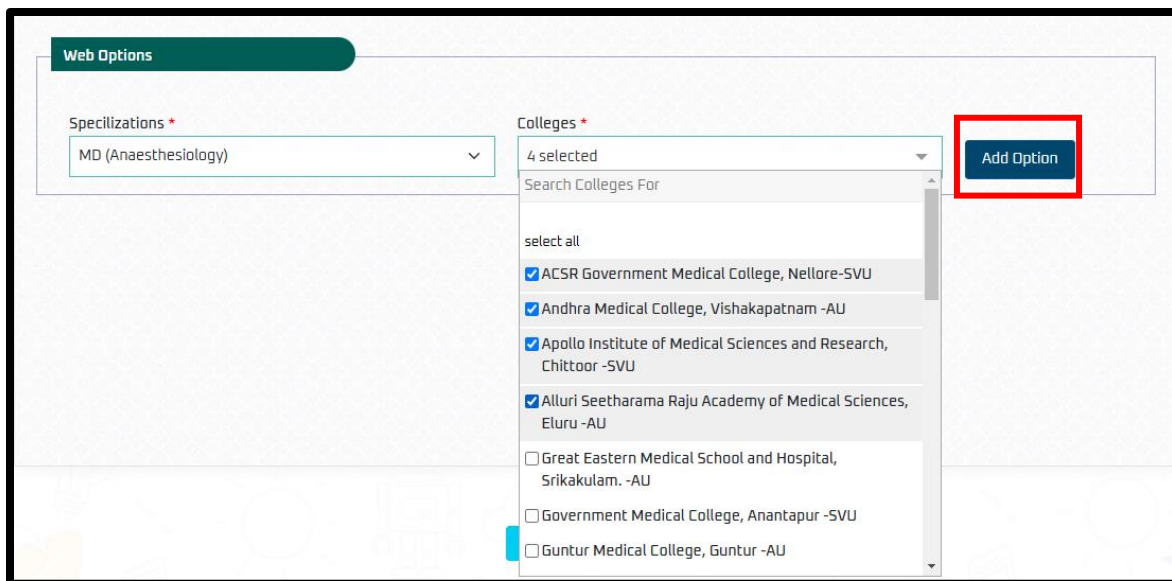
Figure 7: Add Button
